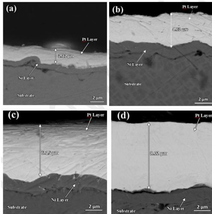
Figure 2: The SEM images of the initial layer of platinum with the approximately thickness of a) 2 \mu m, b) 4 \mu m, c) 6 \mu m and d) 8 \mu m
