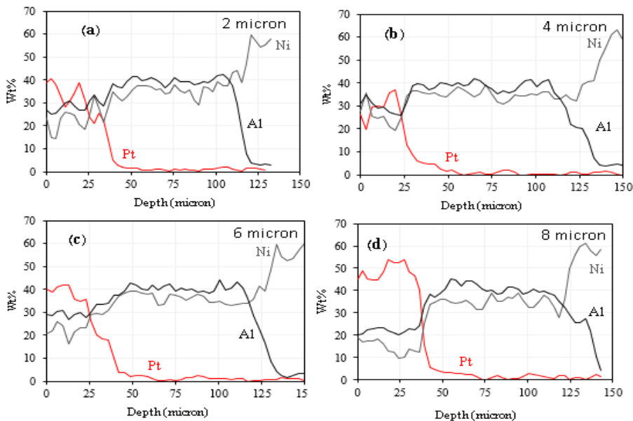
Figure 13: The variation of the concentration and the depth of the diffusion of the Nickel, Platinum and Aluminum in the LTHA for the initial platinum layer with the thickness of a) 2 \mu m, b) 4 \mu m, c) 6 \mu m and d) 8 \mu m
