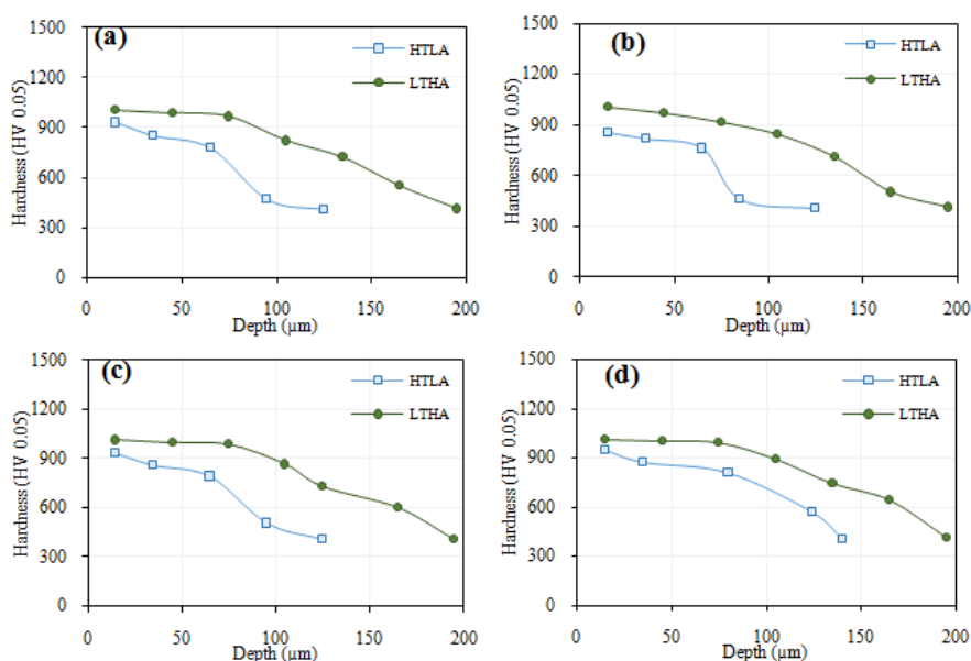
Figure 14: The hardness variation from surface to depth of the Pt-Al coating for HTLA and LTHA methods with the platinum layer with the thickness of a) 2 μm, b) 4 μm, c) 6 μm and d) 8 μm
