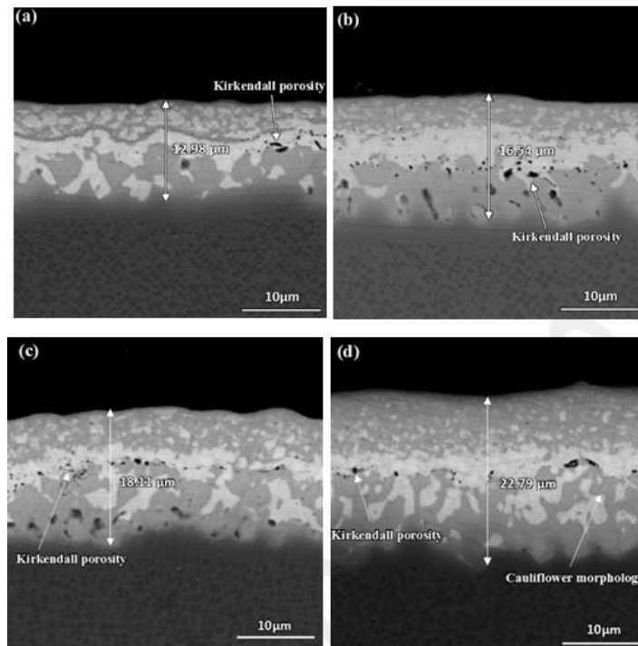
Figure 3: The SEM images of coating after diffusion treatment on the initial layer of platinum with thickness of a) 2 \mu m, b) 4 \mu m, c) 6 \mu m and d) 8 \mu m
