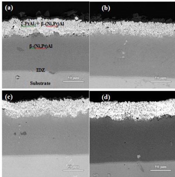
Figure 9: The SEM images of the Pt-Al coating in the LTHA condition for the platinum layer with the thickness of a) 2 \mu\text{m} , b) 4 \mu\text{m} , c) 6 \mu\text{m} and d) 8 \mu\text{m}
