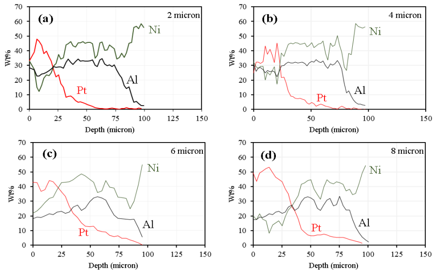
Figure 12: The variation of the concentration and the depth of the diffusion of the Nickel, Platinum and Aluminum in the HTLA for the initial platinum layer with the thickness of a) 2 \mu m, b) 4 \mu m, c) 6 \mu m and d) 8 \mu m
