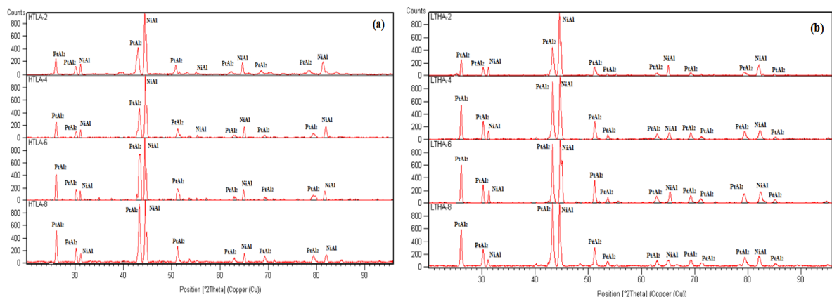
Figure 10: The results of XRD analysis for two methods of a) HTLA and b) LTHA aluminizing process for different thicknesses of initial platinum layer
