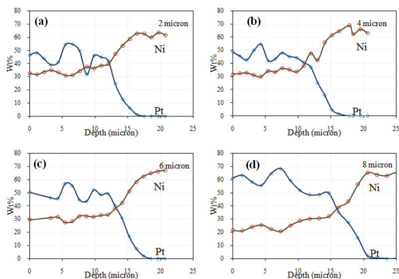
Figure 5: The variations of the concentration and depth of the Ni and Pt diffusion after diffusing treatment of the platinum layer with the thickness of a) 2 \mu m, b) 4 \mu m, c) 6 \mu m and d) 8 \mu m
